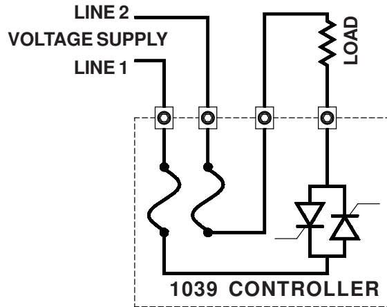
POWER PATH
