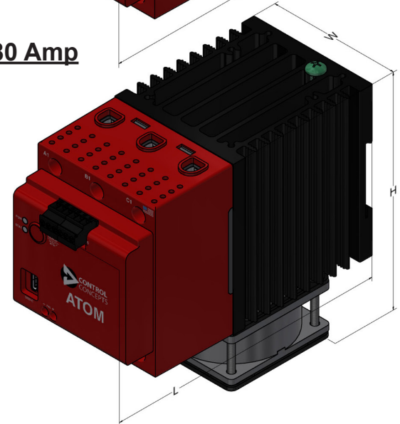
Dimensions: Inches [MM]
